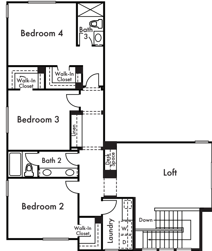
Second Floor
