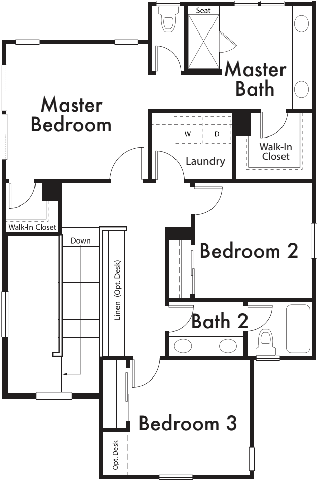
Second Floor
